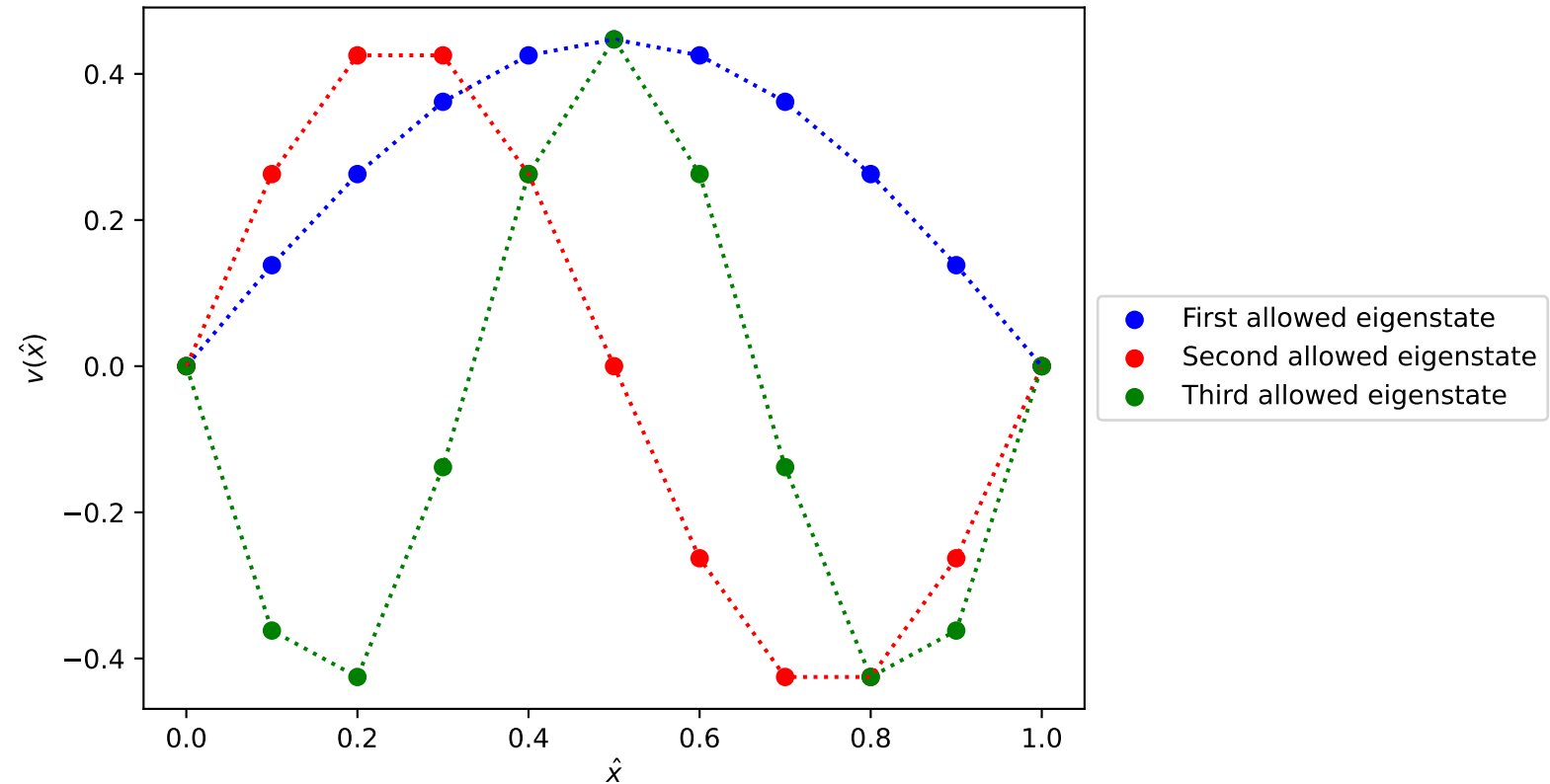
The first three eigenvectors for buckling beam, n=10
